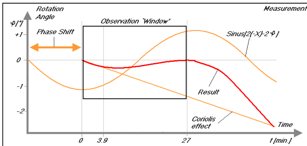
Fig.2) Sketch of a measurement of \varphi versus t with the IGF paraconical pendulum
